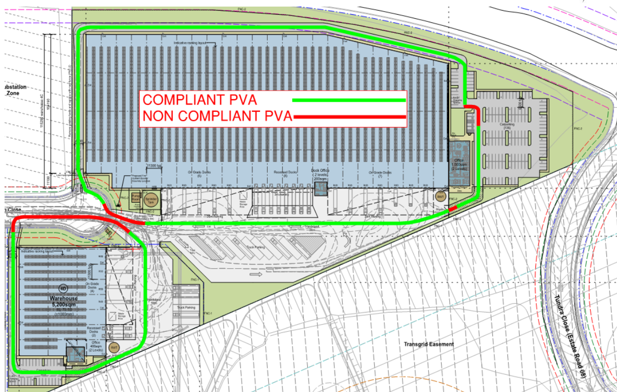
Figure 1 – 4C & 4D Perimeter Vehicular Access per BCA C2.4
